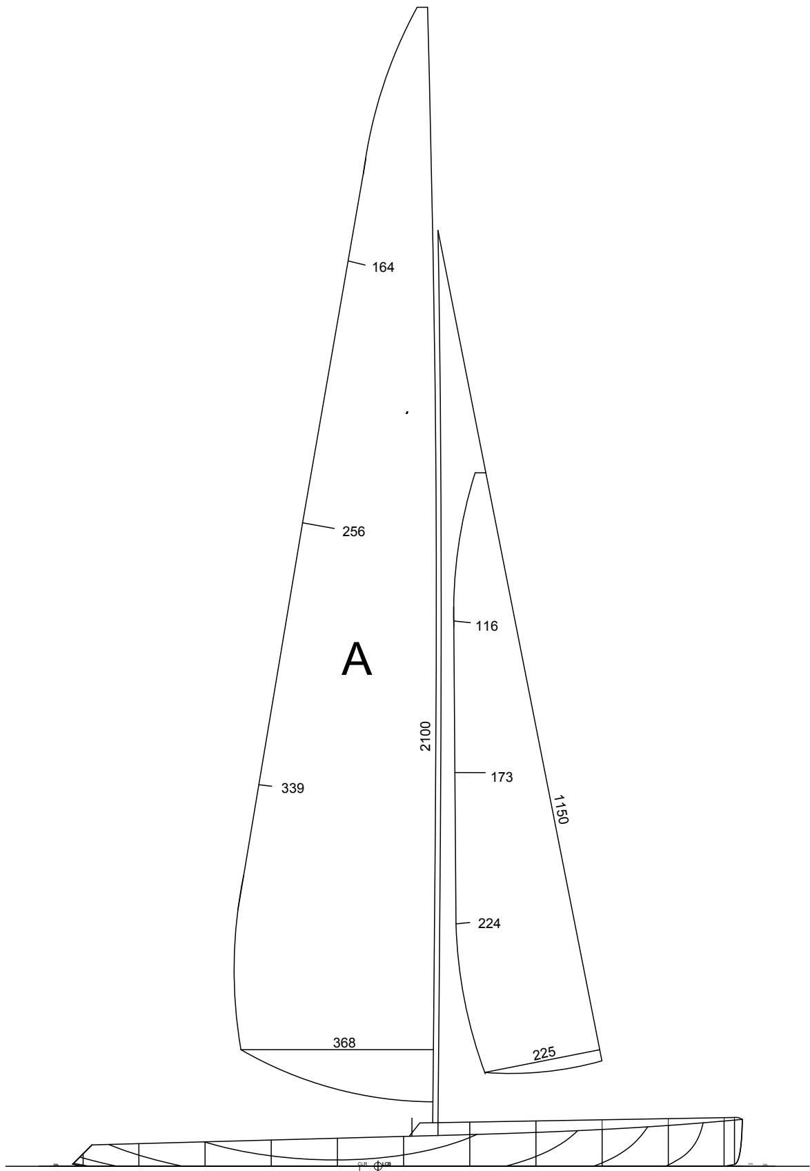
M Class Sail Plans A Rig Swing Scale 1:10 Dwg 1 of 4 191012
