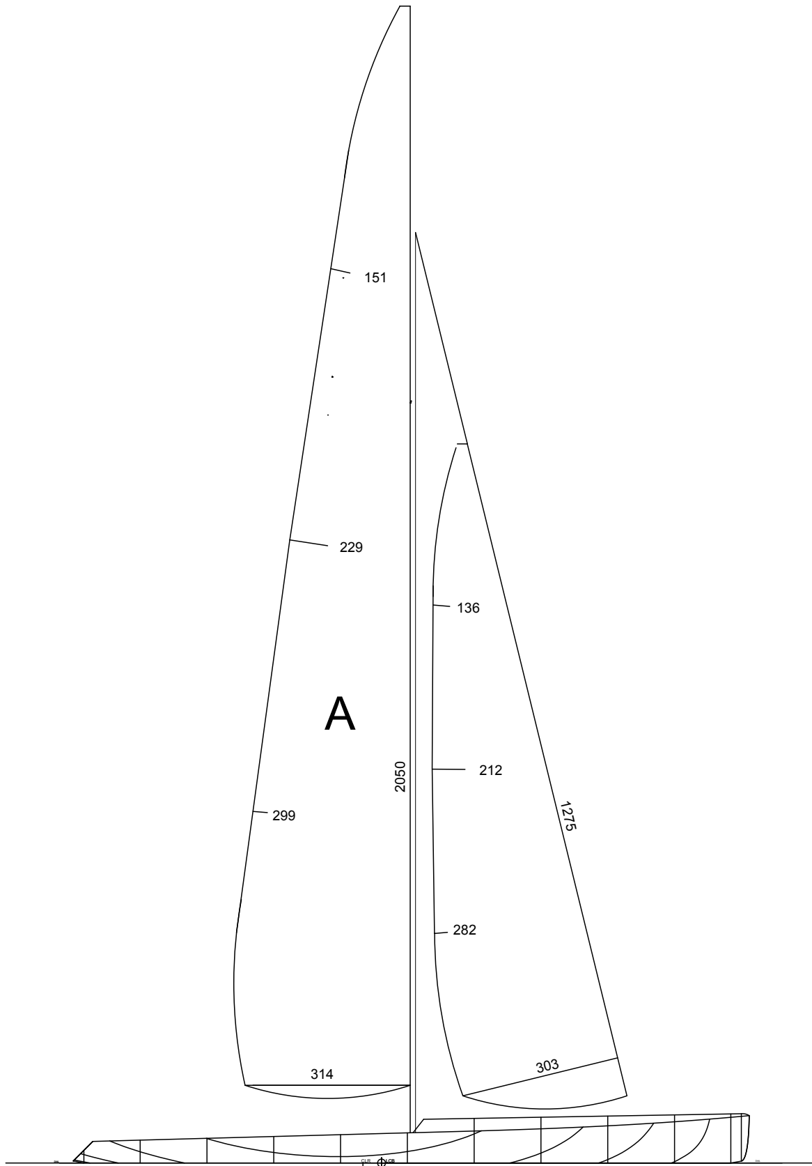
M Class Sail Plans A Rig Conventional Scale 1:10 Dwg 2 of 4 191012
